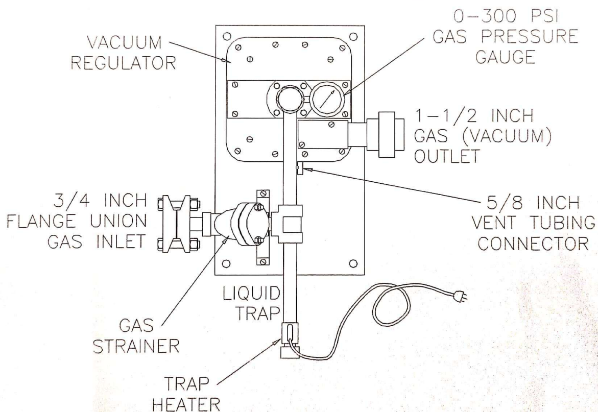
Figure 2 - 8000 PPD (150 kg/h) Vacuum Regualtor Assembly
