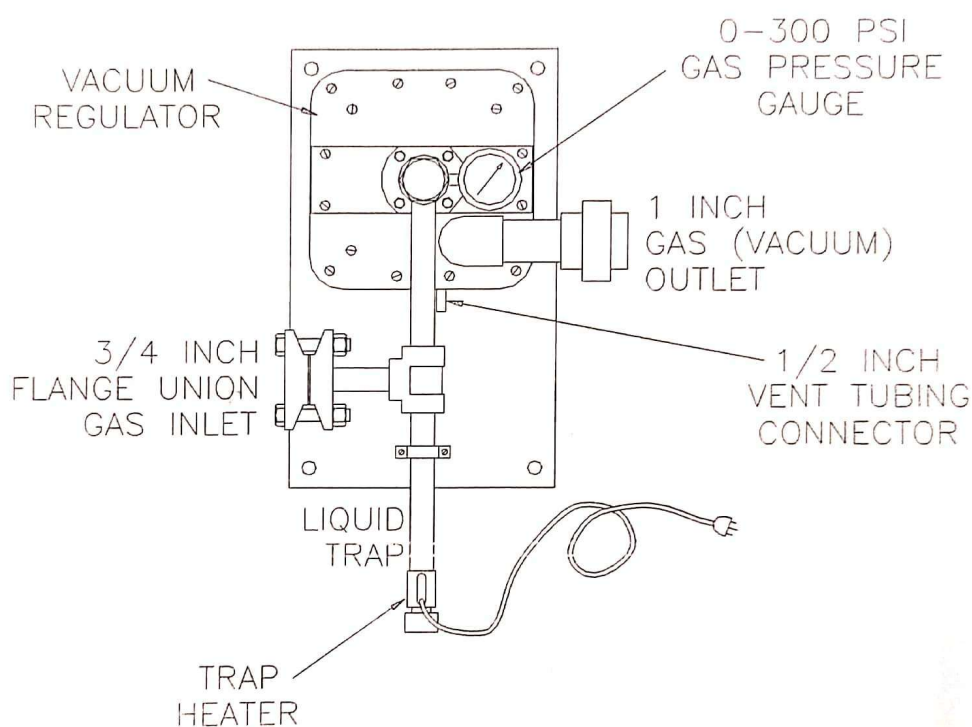
Figure 1 - 2000 PPD (40 kg/h) Vacuum Regulator Assembly
