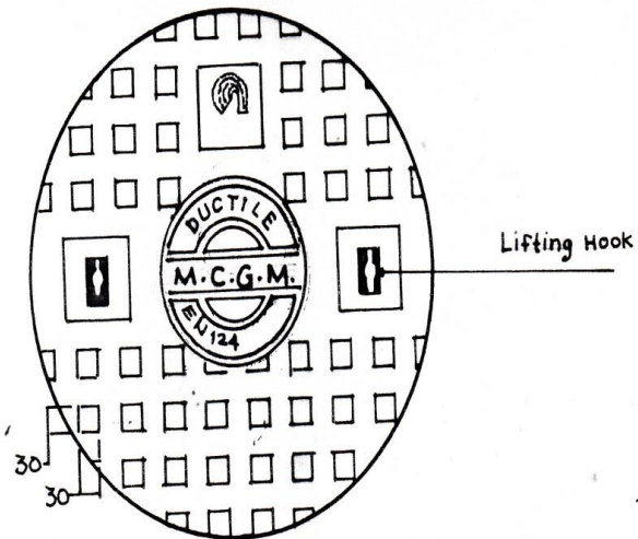
TOP VIEW OF COVER
