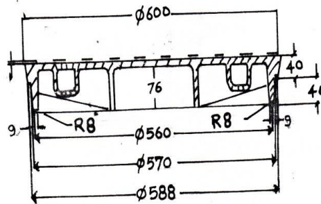
SECTIONAL VIEW OF COVER
